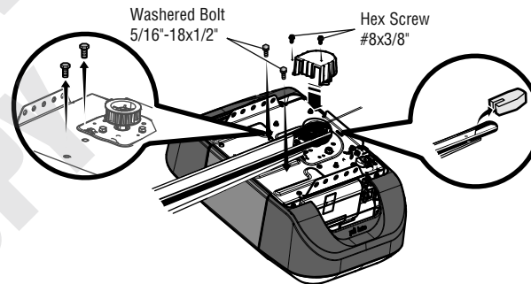
Hex Screw #8x3/8" (Packed with the sprocket cover)
