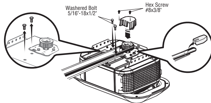
Washed Bolt 5/16"-18x1/2" (Mounted in the garage door opener) (2)
